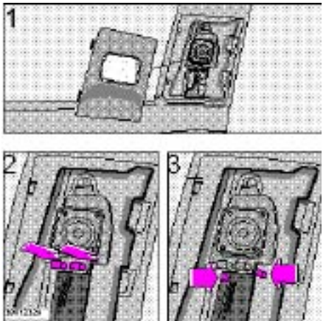
Removing speaker from upper section
